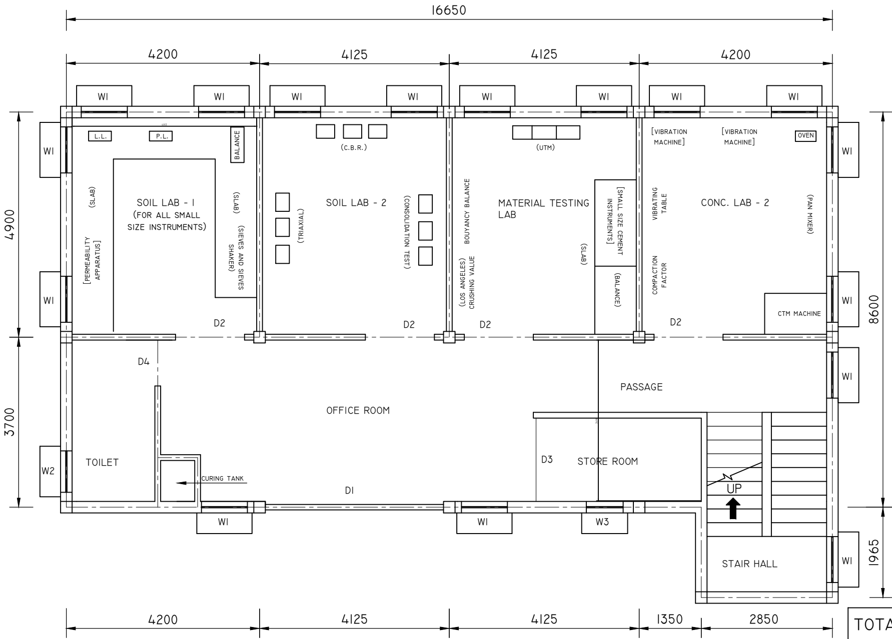
TYPICAL PLAN OF QUALITY CONTROL LABORATORY SCALE - 1 : 100
