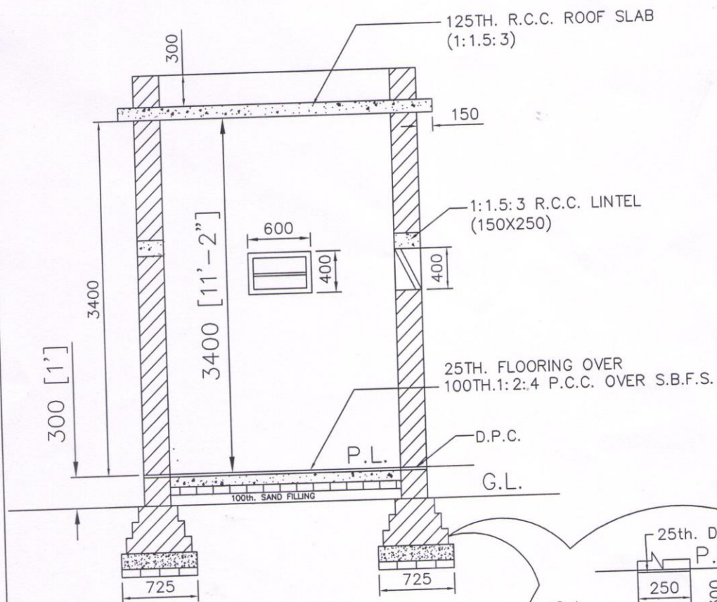
SECTIONAL ELEVATION AT SEC. X-X
